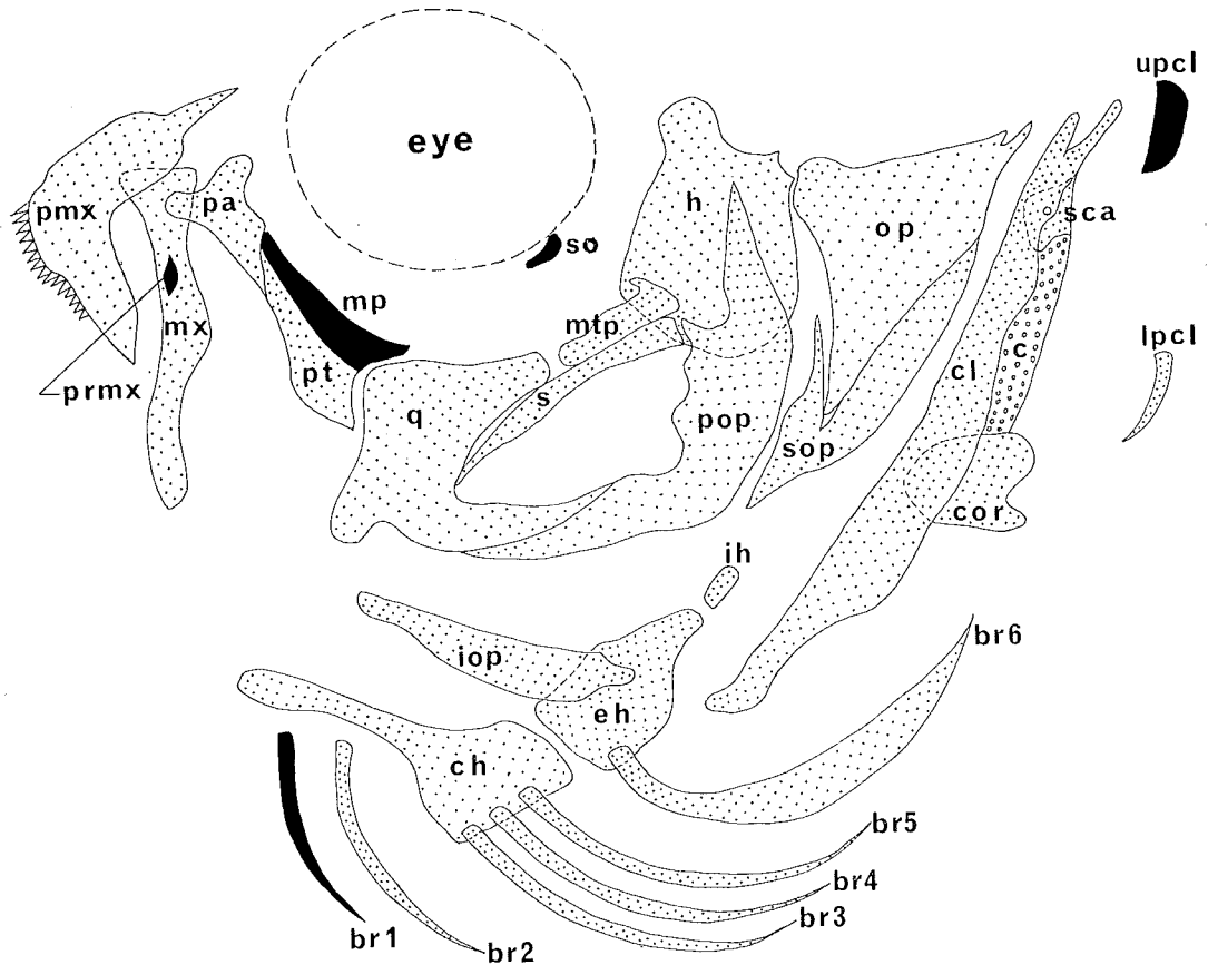
Fig. 7. Comparison of bones of Oxyeleotris marmorata and Callogobius showing the loss of bones (black portions) in the latter. br 1~6, branchiostegals; c, cartilage; ch, ceratohyal; cl, cleithrum; cor, coracoid; eh, epihyal; h, hyomandibular; ih, interhyal; iop, interopercle; lpcl, lower post-cleithrum; mp, mesopterygoid; mtp, metapterygoid; mx, maxilla; op, opercle; pa, palatine; pop, preopercle; pmx, premaxilla; prmx, process of maxilla; pt, pterygoid; q, quadrate; s, symplectic; sca, scapula; so, sub-orbital; sop, subopercle; upcl, upper post-cleithrum.
