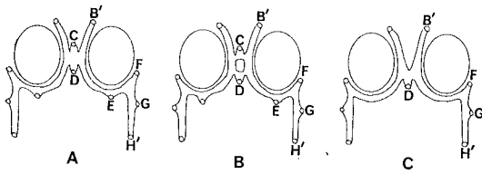
Fig. 5. Three types of anterior oculoscapular canals of Callogobius . A, C. snelliusi , C. sclateri and C. hasseltii ; B, C. okinawae ; C, C. tanegasimae . B'~H', canal pores; ', pore at tip of canal.
