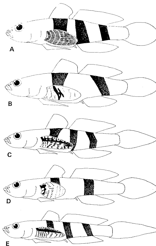
Fig. 4. Diagnostic patterns of five species of Callogobius . A, C. snelliusi (Shunkanhaze); B, C. sclateri (Futasujihaze); C, C. hasseltii (Okinawahaze); D, C. okinawae (Namerahaze); E, C. tanegasimae (Tanehaze).
