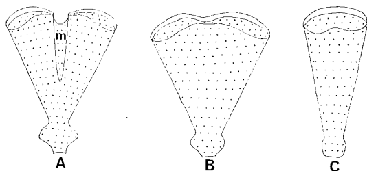
Fig. 3. Ventral views of glossohyal of Callogobius . A, C. snelliusi from Aoyagi collection, 35 mm in standard length; B, C. snelliusi from Aoyagi collection, 31 mm S. L.; C, C. sclateri from AMS I. 17094-03, 33 mm S. L. Stained part stippled. m, membranous part.
